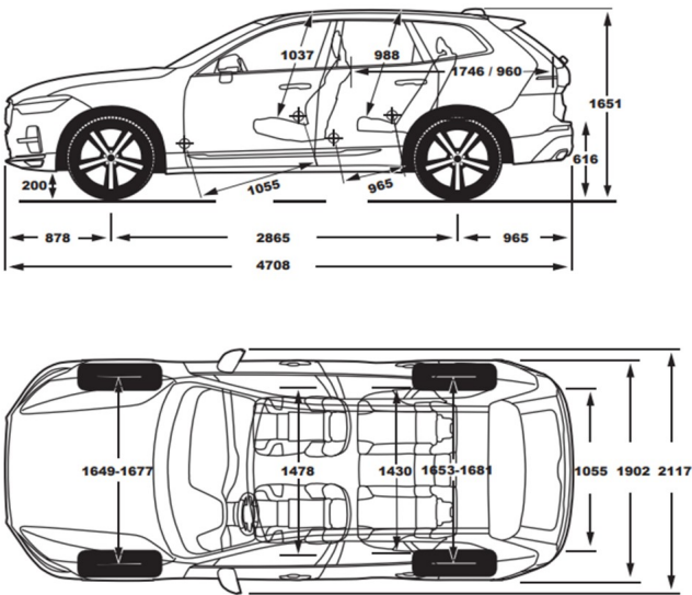
PHEV
